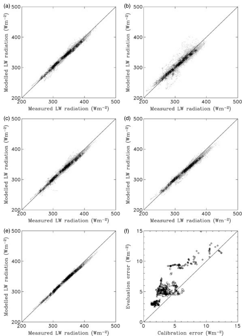
Figure 9. Sub-canopy longwave radiation measured by the five long-term radiometers and modelled by the regression model with a 10-day calibration period. Grey points in (a)–(e) show 15-min averages and black crosses show daily averages. (f) shows evaluation and calibration errors for each possible 10-day calibration period for radiometers 1 (+), 2 ( \diamond ), 3 ( \Delta ), 4 ( \square ) and 5 ( \times ), as listed in Table IV
