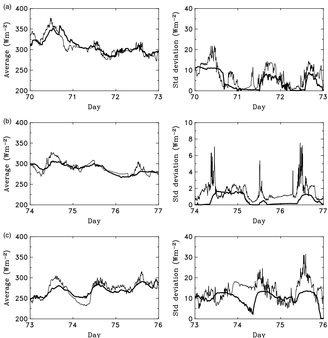
Figure 6. As Figure 5, but for the model using measured sky view and air temperature and modelled above-canopy longwave radiation
