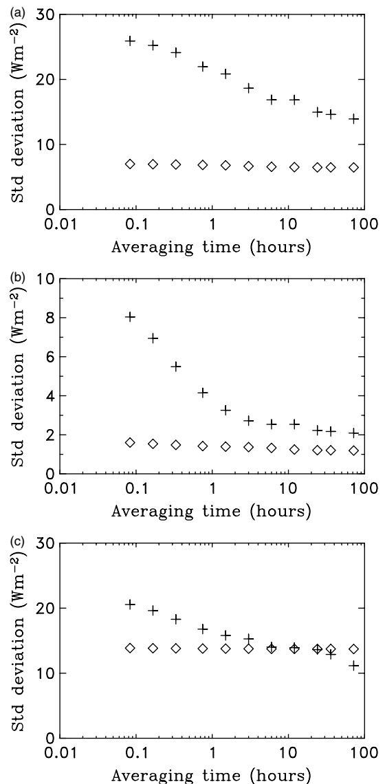
Figure 4. Spatial standard deviations of shortwave (+) and longwave (◇) radiation for varying averaging periods in (a) the southeast-facing forest, (b) the level forest and (c) the forest gap
