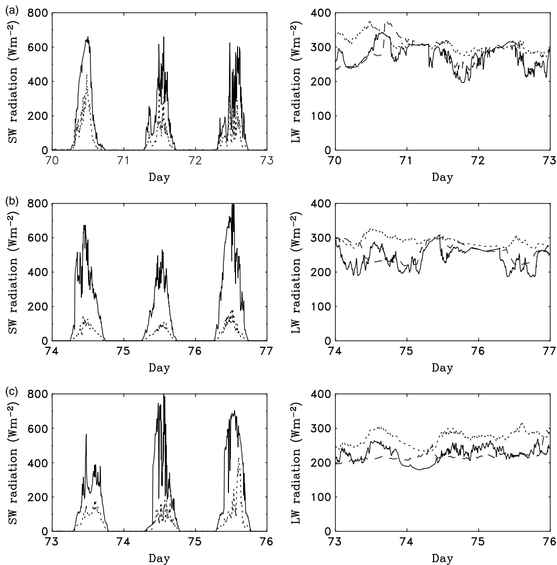
Figure 2. Shortwave radiation (left) and longwave radiation (right) measured above (solid lines) and below (dotted lines) the canopies for the periods that sub-canopy radiometer arrays were deployed in (a) the southeast-facing forest, (b) the level forest and (c) the forest gap. Dashed lines show modelled above-canopy longwave radiation
