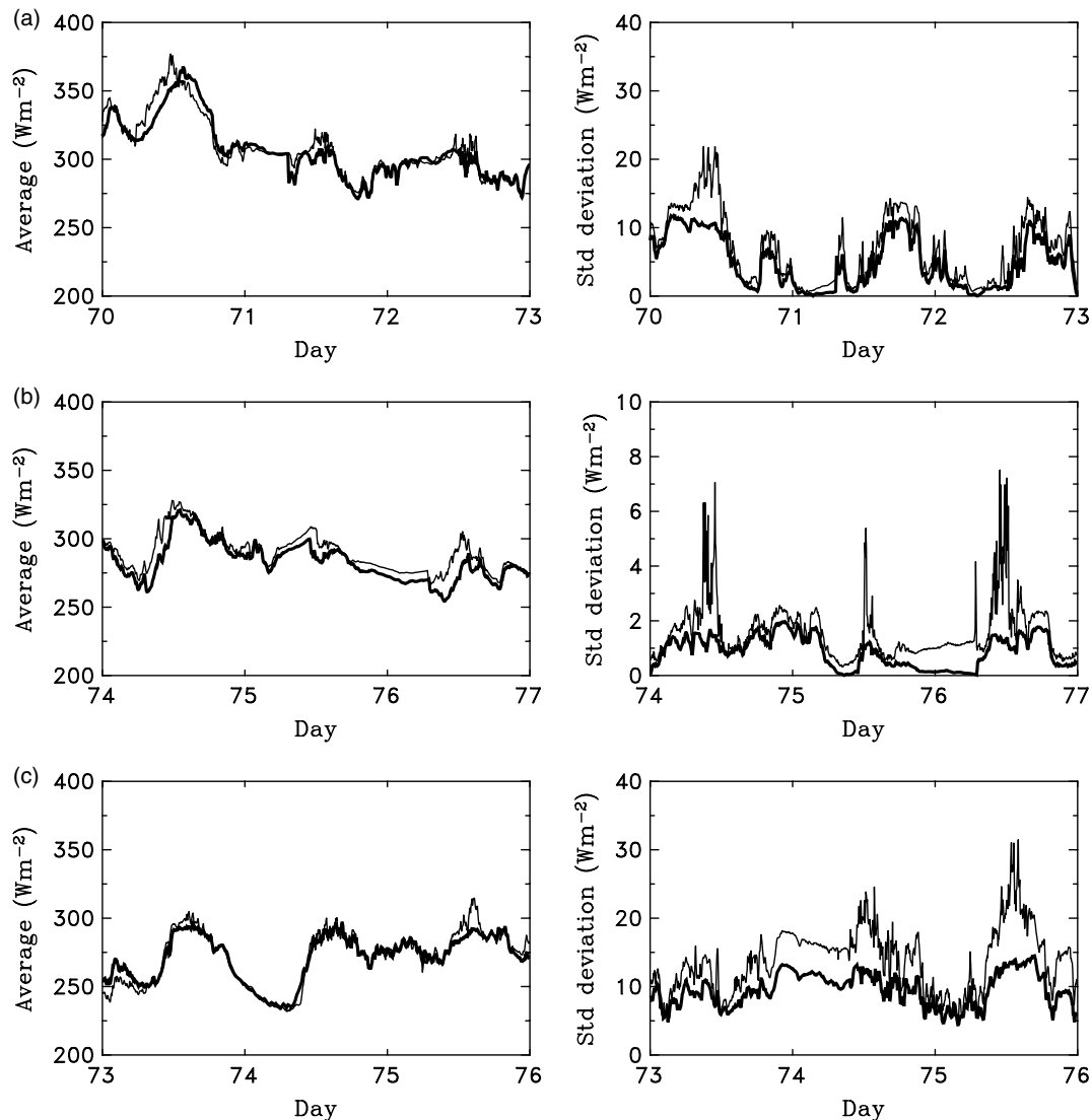
Figure 5. Spatial averages (left) and standard deviations (right) across the radiometer arrays for (a) the southeast-facing forest, (b) the level forest and (c) the forest gap. Thin lines are from measurements and thick lines are from the model using measured sky view, air temperature and above-canopy longwave radiation
