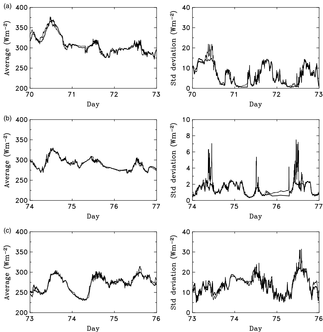
Figure 7. As Figure 5, but for the linear regression model using measured air temperature, above-canopy longwave radiation and above-canopy shortwave radiation
